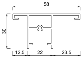
2138658 Stulpprofil 58 mm FB
