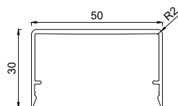
2127030 Abdeckprofil 50 mm, 30 mm, Radius 2 mm
