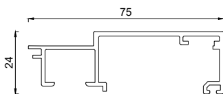
2141175 Rahmen 75mm FVNG IN
