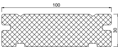
3952100 SE-Pad 30 x 100 mm
