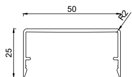
2127025 Abdeckprofil 50 mm, 25 mm, Radius 2 mm
